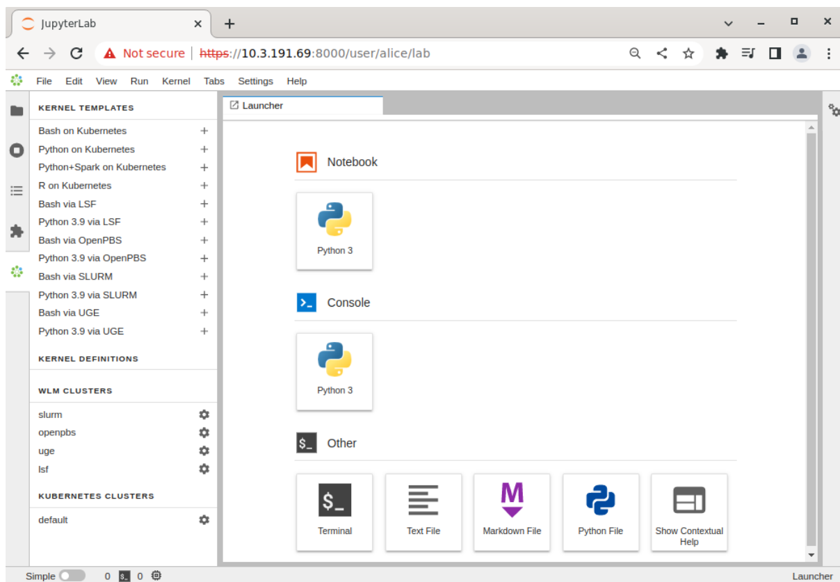
Figure 13.2: JupyterLab Bright extensions section with kernel templates
