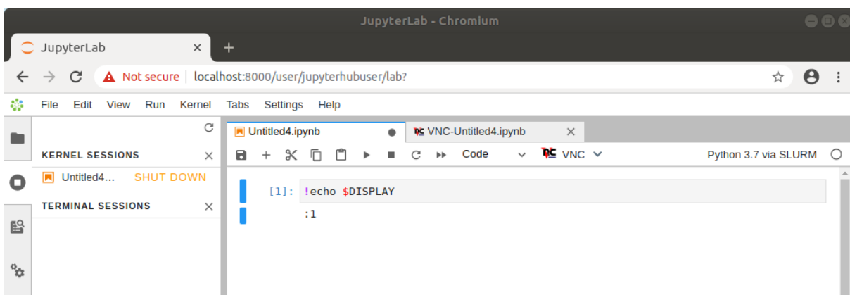
Figure 13.10: Automatic configuration of DISPLAY environment variable
