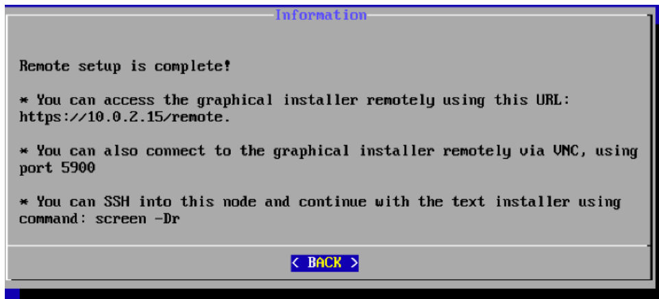
Figure 3.26: Ncurses Remote Installation Remote URL Displayed
