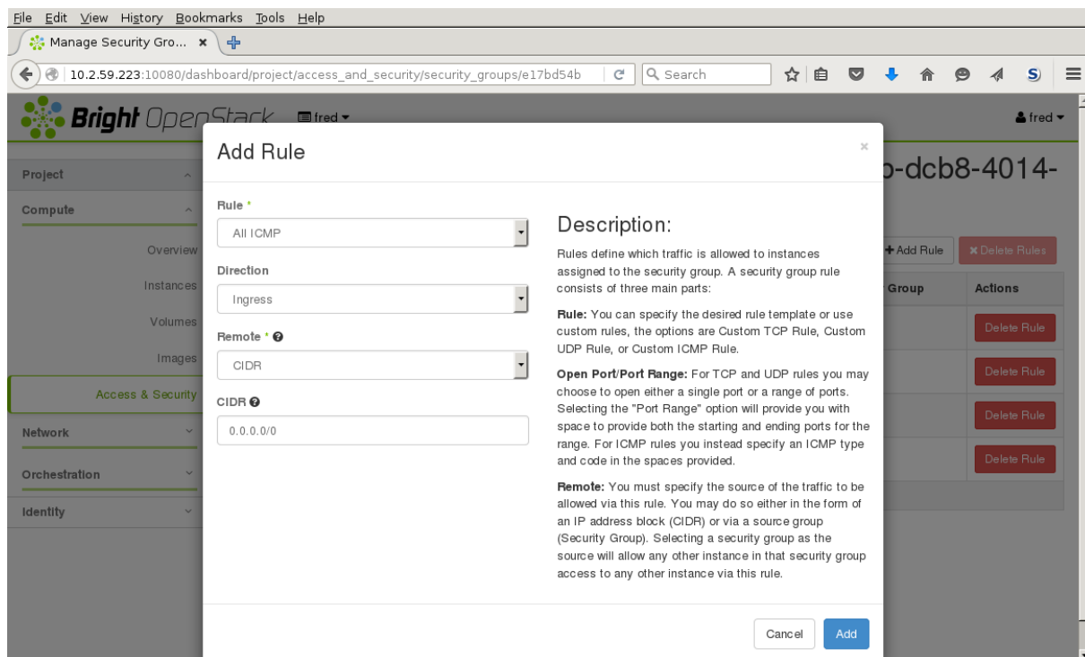
Figure 15.12: Security Group Rules Management—Adding A Rule
