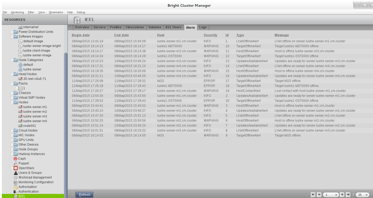
Figure 7.29: IEEL Alerts
