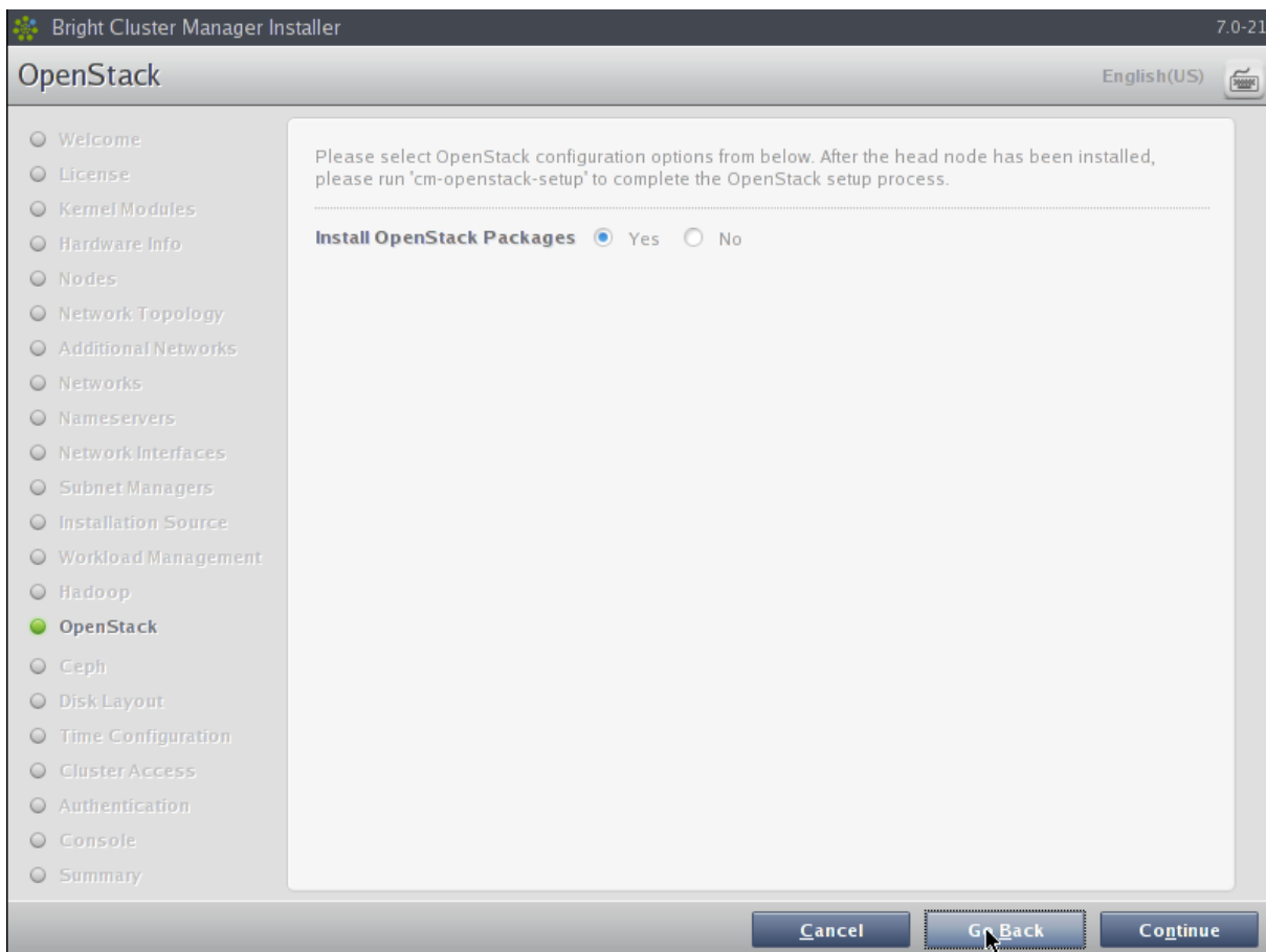
Figure 3.23: OpenStack Option
