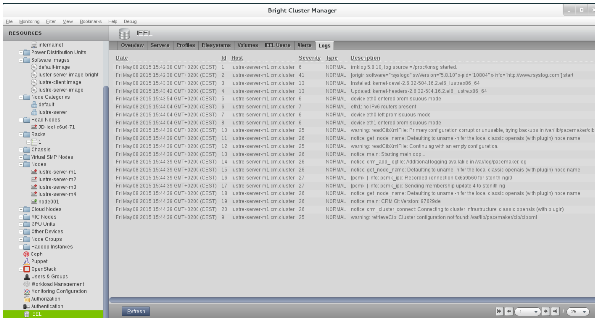
Figure 7.30: IEEL Logs
