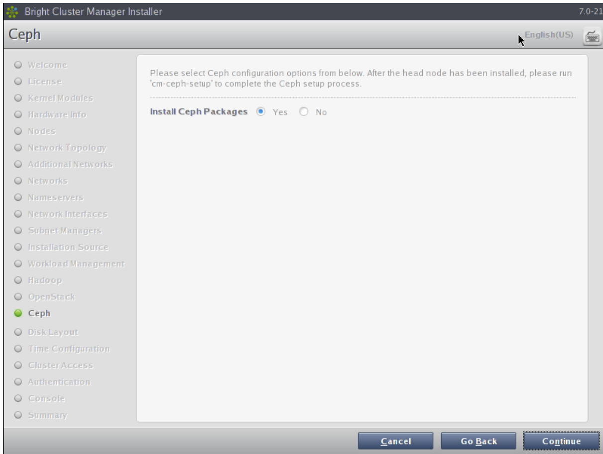
Figure 3.24: Ceph Option
