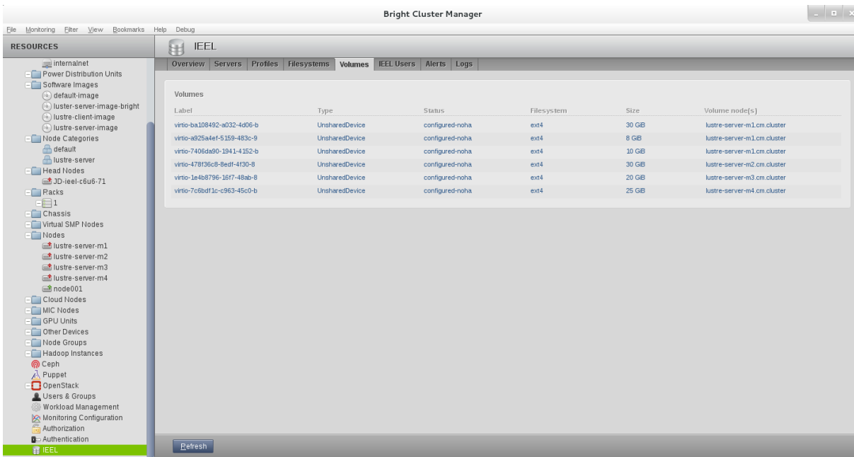
Figure 7.27: IEEL Volumes
