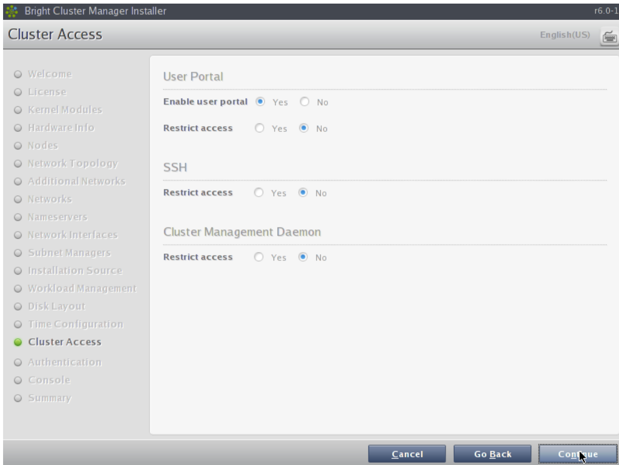
Figure 3.28: Cluster Access
