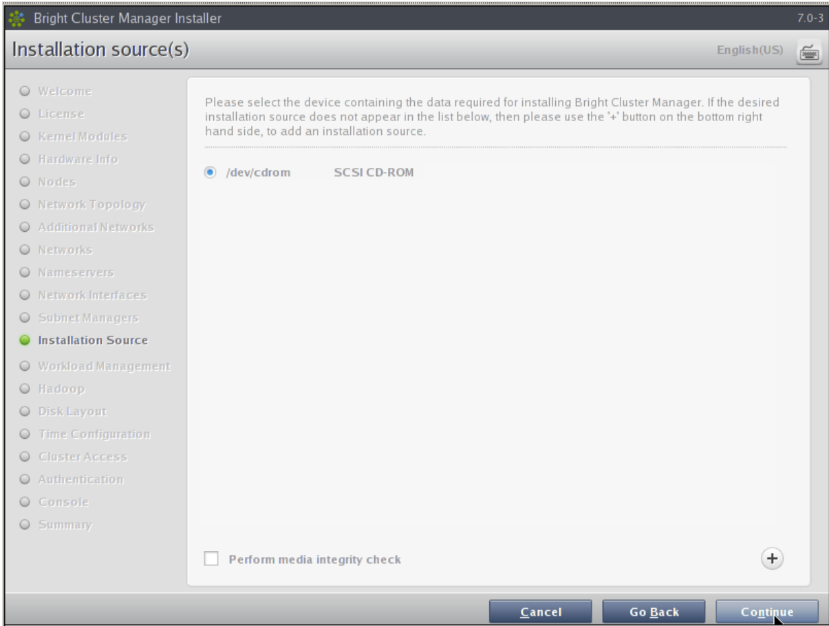
Figure 3.20: DVD Selection
