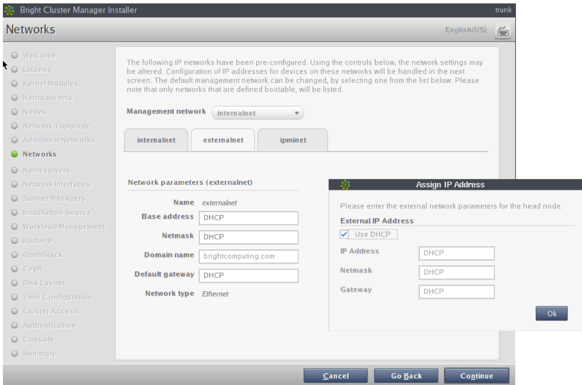
Figure 3.15: Networks Configuration
