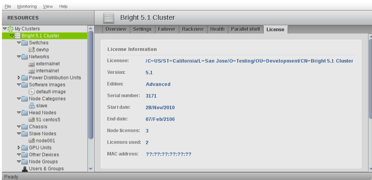
Figure 4.1: License Information
