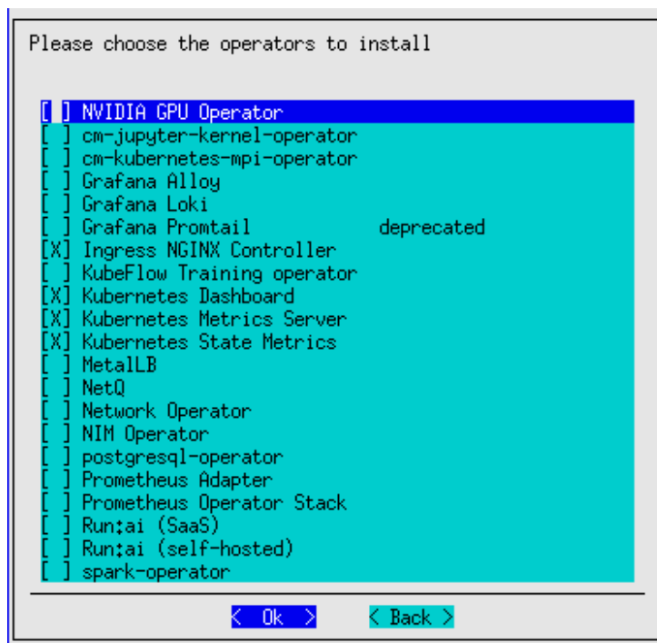
Figure 6.1: Kubernetes setup TUI session: selection of operator packages to be installed
